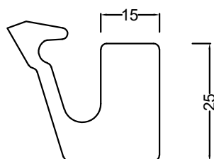
Piston Seal
